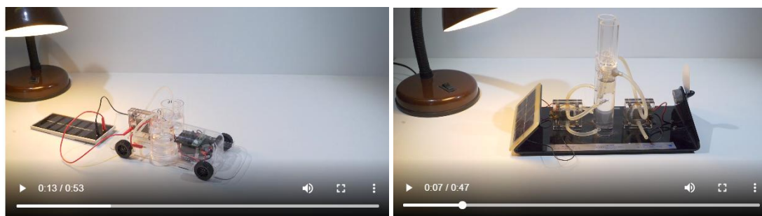
Fig. 30 Comparison of two experimental set ups with FCH used on workshops in secondary schools: (a) Horizon kit, with a detachable photovoltaic cell, connected here to the fuel cell mounted on a toy car. (b) Thames-Cosmos set up, with the PV cell mounted permanently and connected to FCH used as electrolyser; in the middle – containers for H_2 and O_2 (with vertical scale signed); to the right – a second FCH used to produce the electrical current that in turn is supplied to a small electrical motor moving a fan. (Source: UMK)
