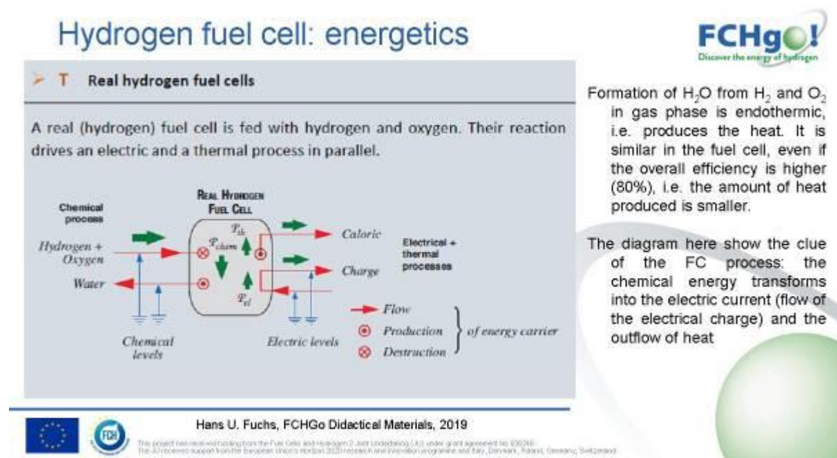
Fig. 31. Three complementary pictures how the hydrogen fuel cell works: the historical discovery (William Grove), the principle of construction (picture by G. Karwasz); thermodynamics of FCH (H. Fuchs).
