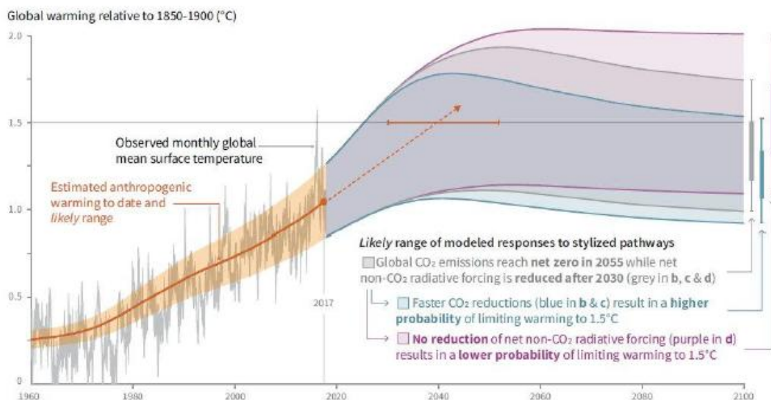
Fig. 4. The most important result of the latest IPCC report on climate change: the expected temperature increase (relative to the pre-industrial era) will be around 1-2°C (depending on the CO 2 emission scenarios) and will reach a maximum around 2050. The model assumes reducing CO 2 emissions to zero in 2055. Source: [4]
