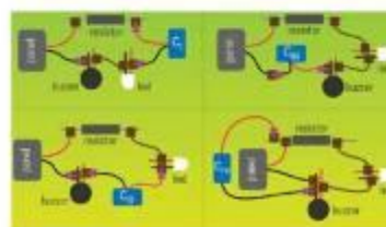
Figure 12: 5-load circuit for 4 currents
