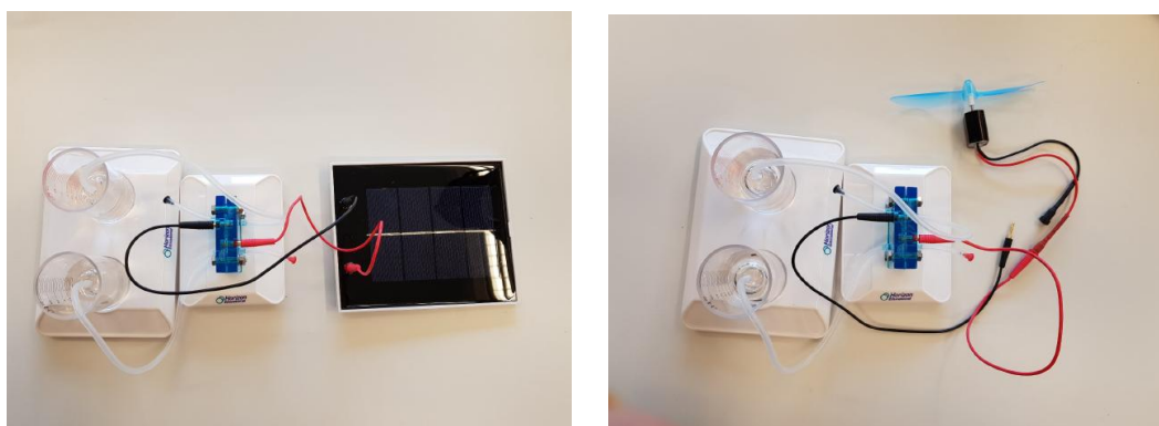
Fig. 3: Experiment At ZHAW for 4th form of elementary school: (a) electrolysis of water in a reversible fuel hydrogen cell in using “electricity from a photovoltaic panel; (b) using the hydrogen and oxygen produced to generate electricity in FHC and supply the current to a small fan. (photo E. Dumont).
