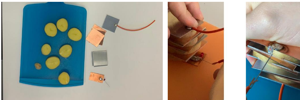
Fig. 2. FCHgo workshop at ZHAW foe Winthertur elementary school: building potato battery; (a) material prepared for pupils; (b) & (c) ready construction: that in the middle does not work, as the order of Cu/Zn pairs is mixed; the pile to the right is build correctly and the LED lit up.
