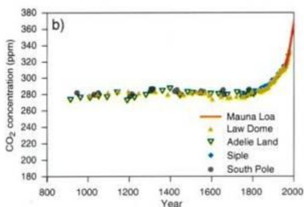
Fig. 19. Historical changes in \text{CO}_2 content in the Earth's atmosphere (Source: Scripps Institution of Oceanography)
